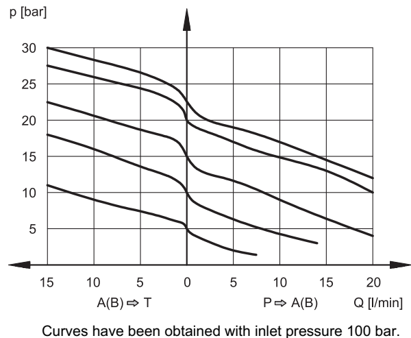
PRESSURE VARIATION p=f(Q)
