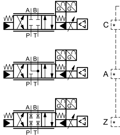
detailed symbol (spool Z)
