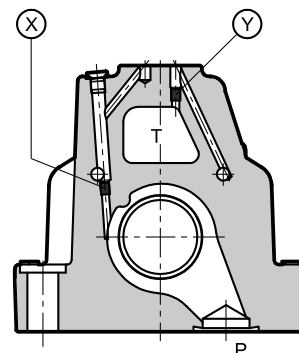
DXRE10J/DXRE11J
