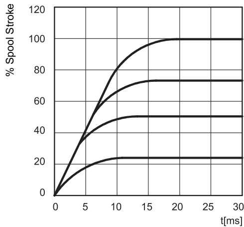
STEP RESPONSE
