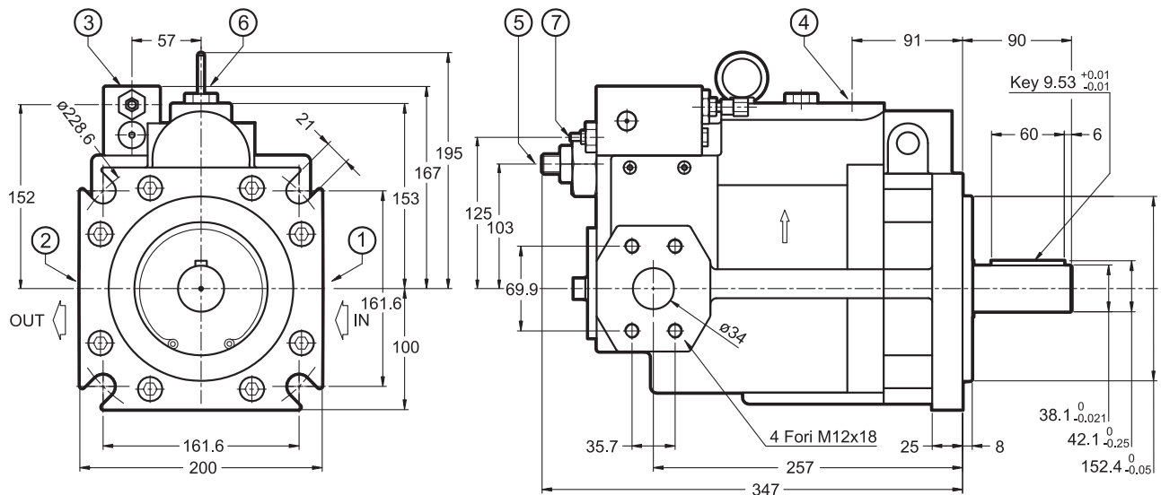
VPPL-100PC6 PUMP
