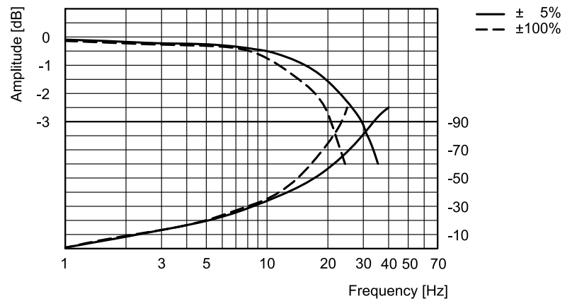
FREQUENCY RESPONSE
