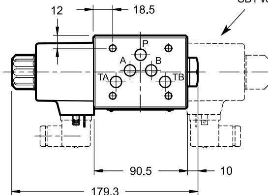
MDS5-TA/10*-D*
